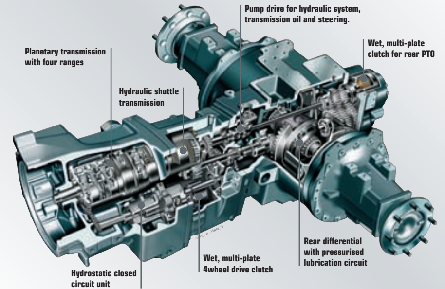
Agrotion TTV 620 drive train.
