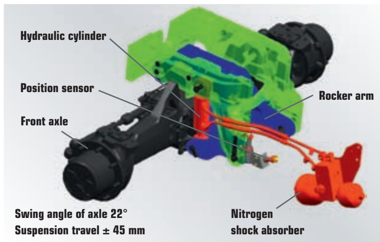
Comfortable and safe: The Agrottron TTV has hydro-pneumatic front axle suspension.
