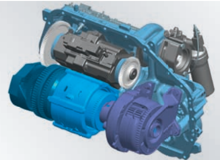
Mechanical-hydraulic drive unit in the Agrotion TTV 630.
